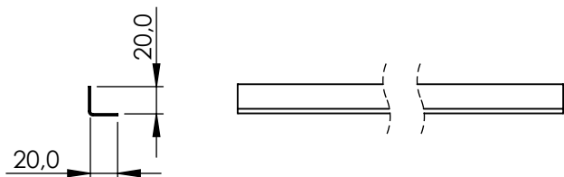
Cantoneira - 3000mm
